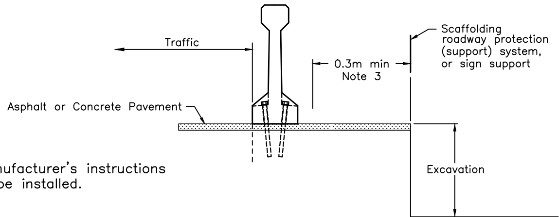
LAYOUT ADJACENT TO EXCAVATIONS OR FIXED OBJECTS
