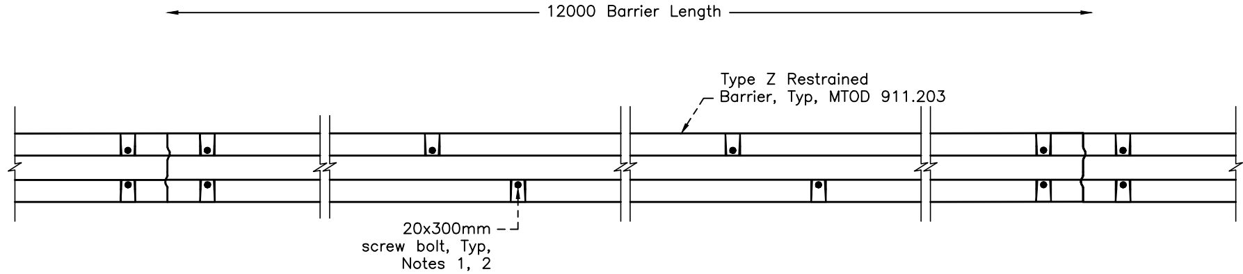
PLAN
